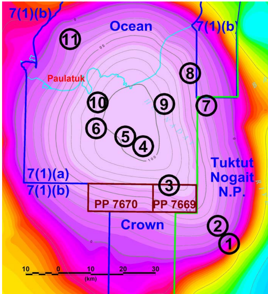
Plan view of Darnley Bay Gravity Anomaly (130 mGal), with the 11 priority gravity targets and the new Prospecting Permits PP 7669 and PP 7670 (awarded February 1, 2009).
