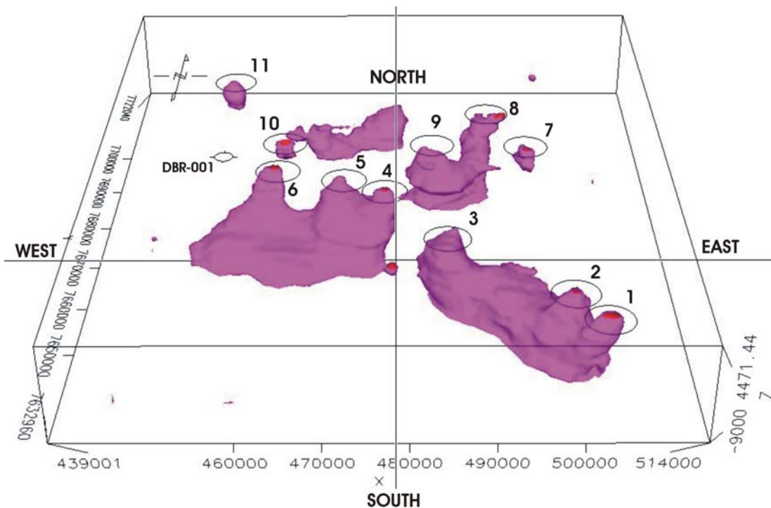
3D model of the highest density sources, with the 11 priority gravity targets.
